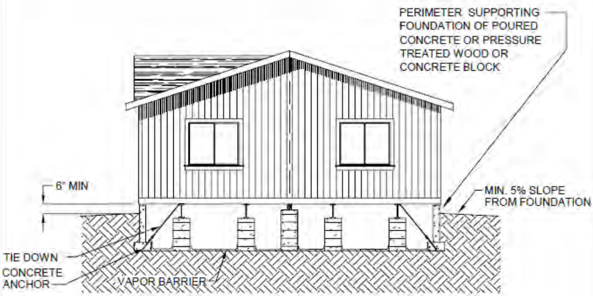
PERMANENT FOUNDATION SET FIGURE 301.2
